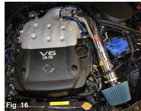
Fig 16 The cold air intake is seen in this picture used as a short ram.
