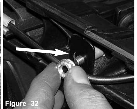
Figure 32 The m6 flange nut is used to tighten the reservoir bracket in place. Note: The 3/16" spacer between the bracket and cross member, used to support the bracket to keep it from distorting.
