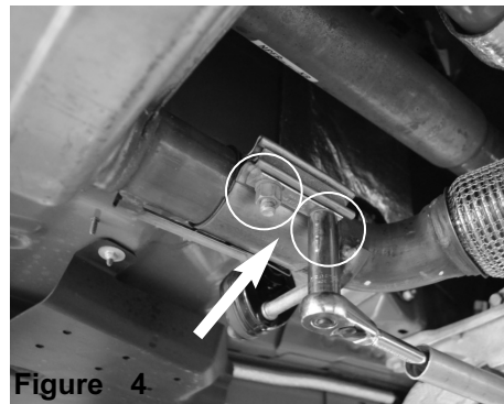
Figure 4 Loosen the 2 15mm nuts on the band clamp on OEM down pipe. Loosen and pull back.
