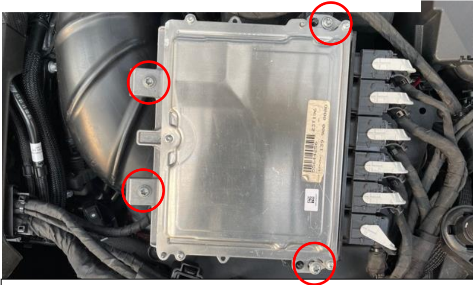
1. Remove the 4 screws holding the ECU down.
