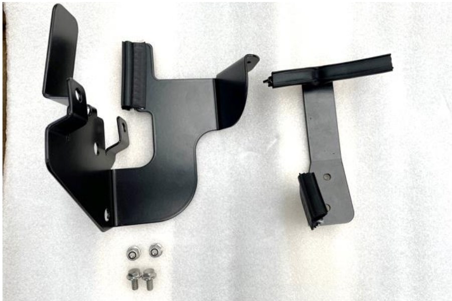
11. Take the 2 supplied brackets, 2 x Lock Nuts and 2 x M6x16 bolts.
