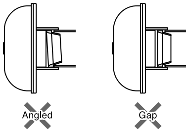
Air Guide Mounting
