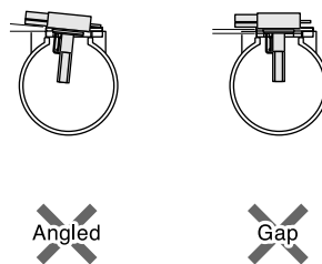
Airflow Meter Sensor Mounting
